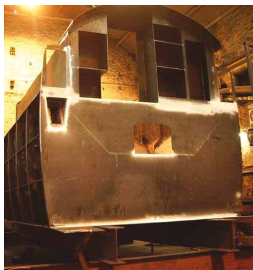
New 5500 Gallon Tender Tank Fabrication for Locomotive No:34092 "City Of Wells". Manufactured against original drawings from the National Railway Museum
